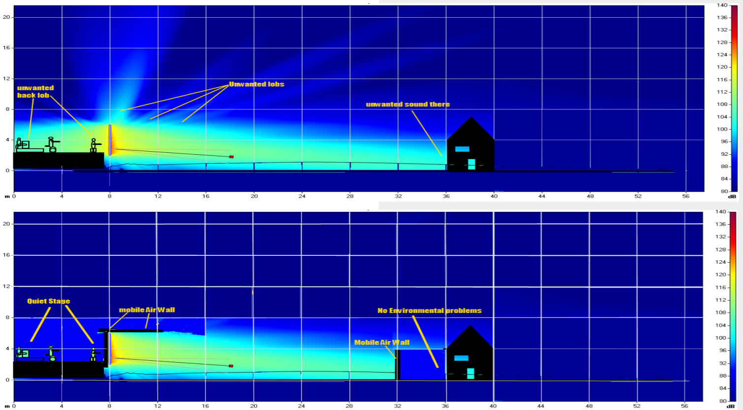
Mobile Air Wall example
